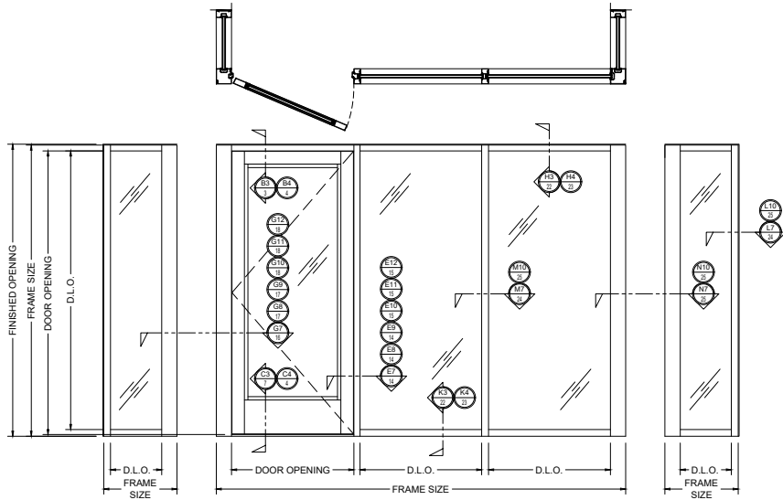
3B) FHC 200 SERIES OFFSET-HUNG ELEVATION
