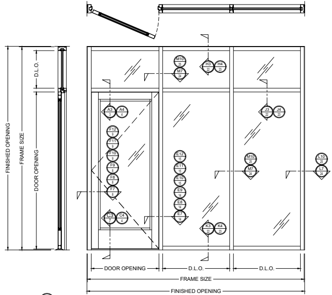
1B) FHC 200 SERIES OFFSET-HUNG ELEVATION
