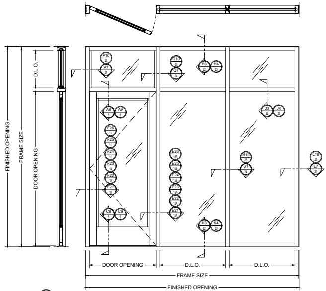
1E FHC 200 SERIES CENTER-HUNG ELEVATION
