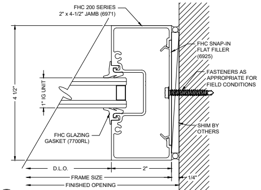
L7 SIDELITE JAMB @ WALL
