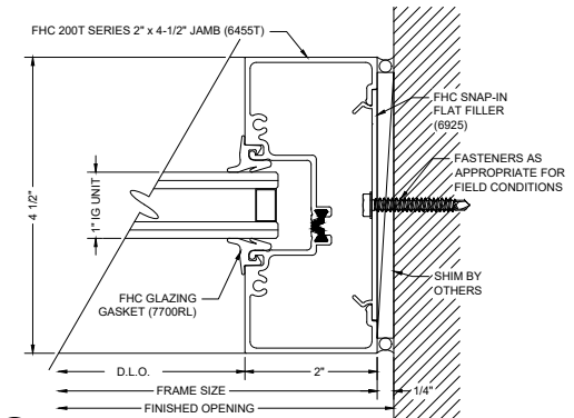
L13 SIDELITE JAMB @ WALL
