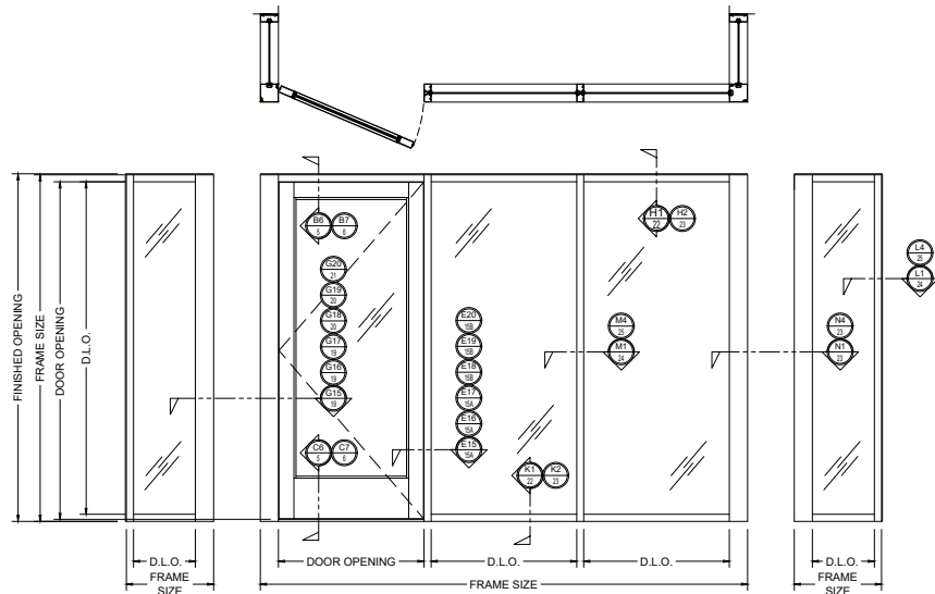
3D FHC 100 SERIES CENTER-HUNG ELEVATION
