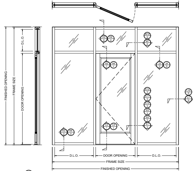
2B) FHC 200 SERIES OFFSET-HUNG ELEVATION
