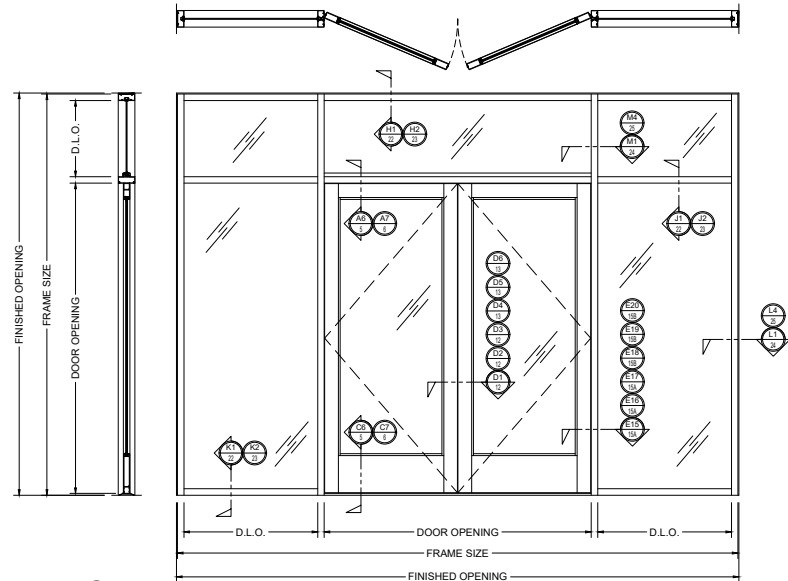
4D FHC 100 SERIES CENTER-HUNG ELEVATION
