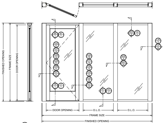
5D FHC 100 SERIES CENTER-HUNG ELEVATION
