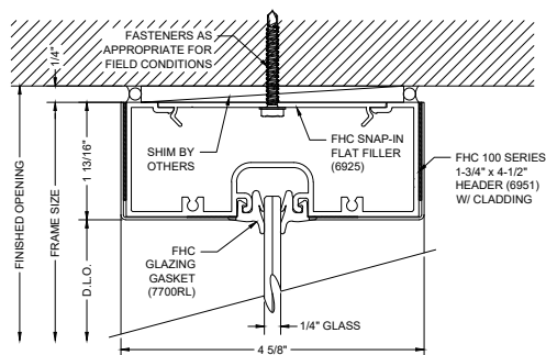
H2 HEADER @ CEILING
