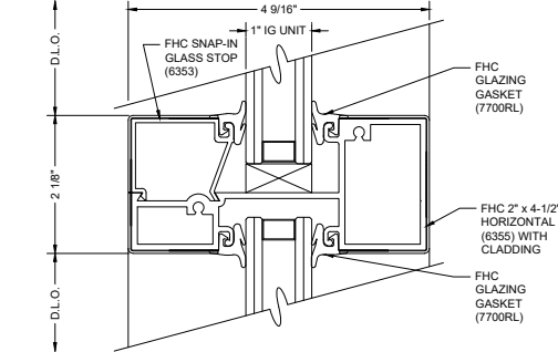
J4 INTERMEDIATE HEADER
