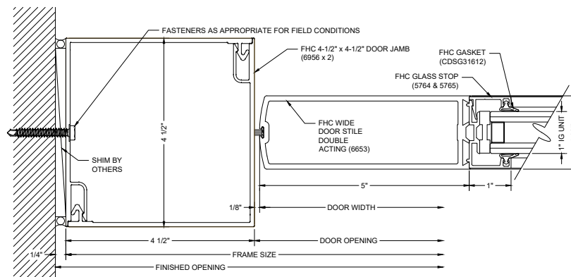
G35 DOOR JAMB @ WALL
