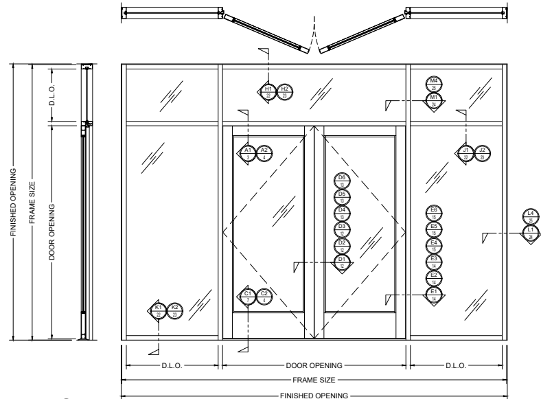
4A FHC 100 SERIES OFFSET-HUNG ELEVATION
