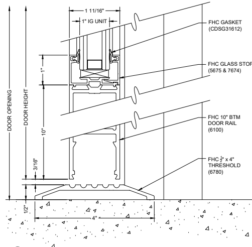
C3 BOTTOM OF DOOR
