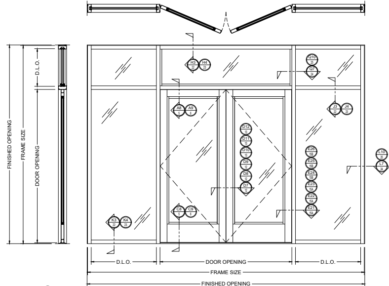
4E FHC 200 SERIES CENTER-HUNG ELEVATION
