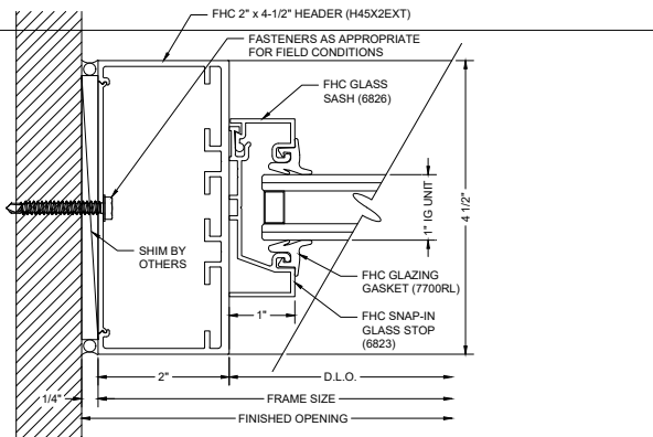
P7 JAMB @ TRANSOM
