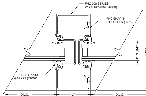
M7 INTERMEDIATE JAMB
