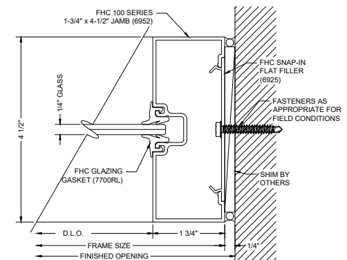
L1 SIDELITE JAMB @ WALL
