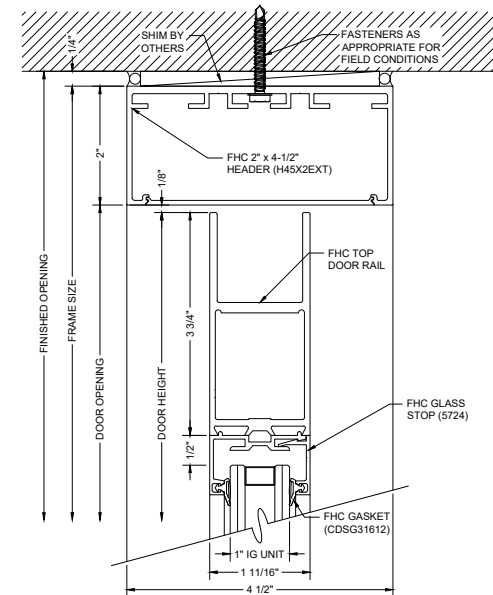
B8 DOOR HEADER
