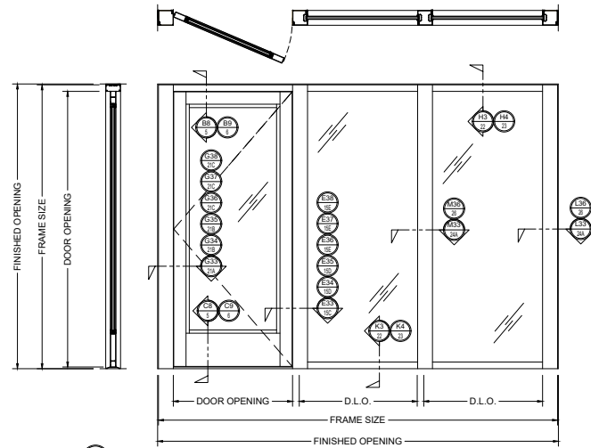
5E FHC 200 SERIES CENTER-HUNG ELEVATION
