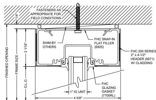
H4 HEADER @ CEILING
