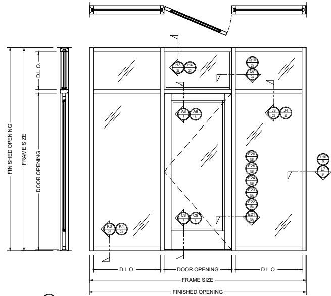
2E FHC 200 SERIES CENTER-HUNG ELEVATION
