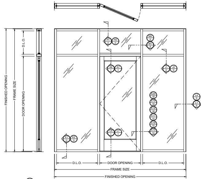
2D FHC 100 SERIES CENTER-HUNG ELEVATION
