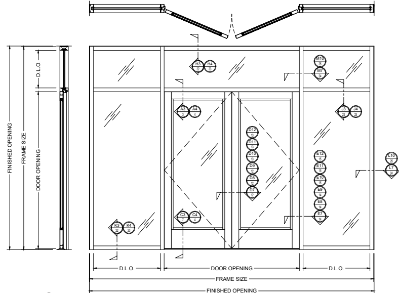
4B) FHC 200 SERIES OFFSET-HUNG ELEVATION
