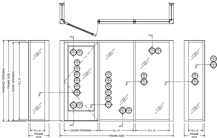
3A FHC 100 SERIES OFFSET-HUNG ELEVATION
