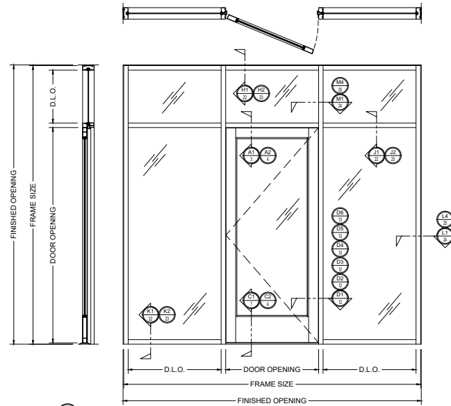
2A FHC 100 SERIES OFFSET-HUNG ELEVATION
