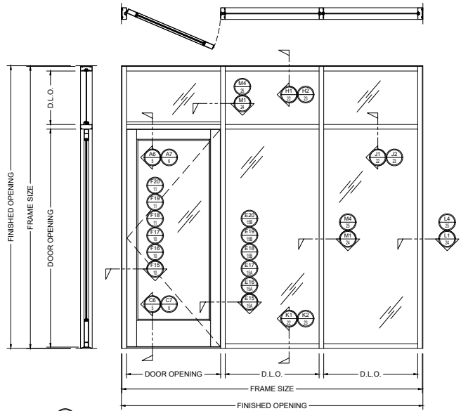
1D FHC 100 SERIES CENTER-HUNG ELEVATION
