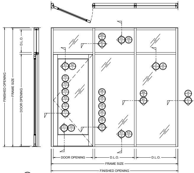
1A FHC 100 SERIES OFFSET-HUNG ELEVATION
