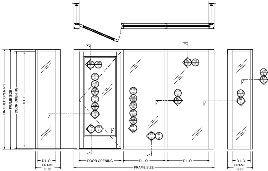
3E FHC 200 SERIES CENTER-HUNG ELEVATION
