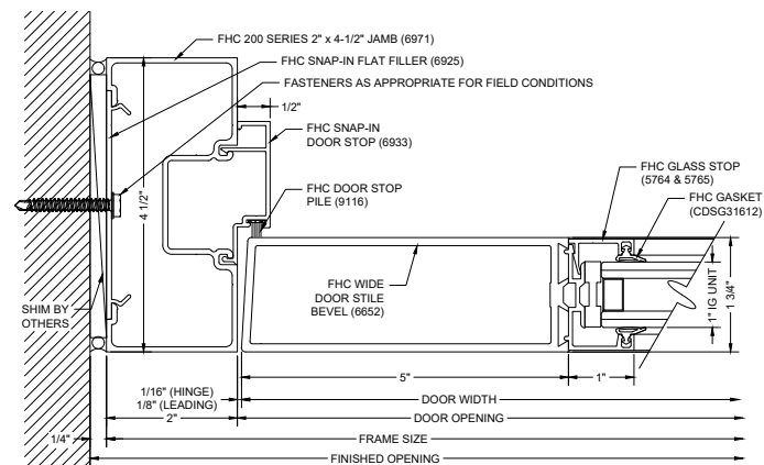
F9 DOOR JAMB @ WALL
