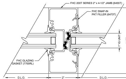
M13 INTERMEDIATE JAMB
