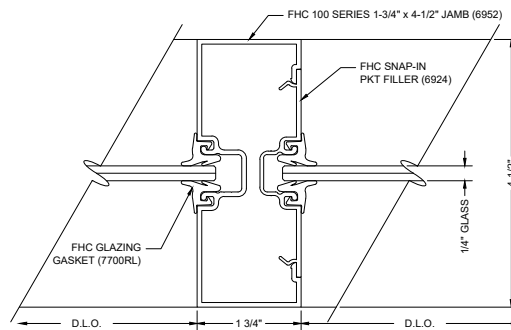
M1 INTERMEDIATE JAMB
